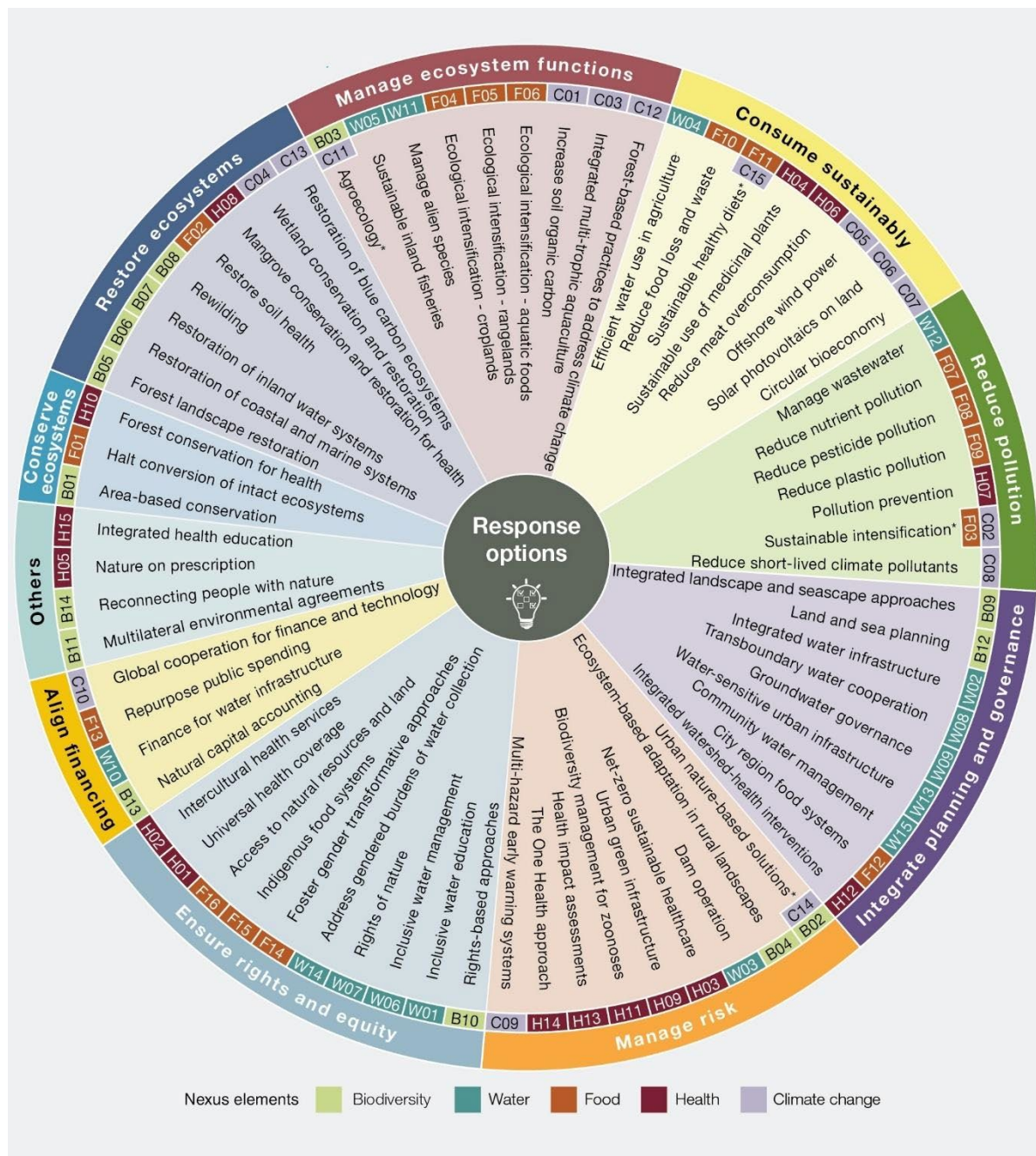
Figure SPM.7. Many response options already exist that a range of actors can implement. The 71 response options assessed in chapter 5 are displayed as wedges and are grouped into 10 broad categories of actions (labelled on the outer edge of circle). Unique alphanumeric codes for each response option indicate its nexus element (B for biodiversity, W for water, F for food, H for health and C for climate change) and unique number. These codes are used to identify response options throughout the report. For brief descriptions of response options, see Appendix IV. Several response options correspond to more than one category but, for clarity, are displayed only in their primary category. The “Others” category includes four important response options that do not correspond easily to the nine main categories. Response options with an asterisk (agroecology, sustainable healthy diets, sustainable intensification and urban nature-based solutions) each were assessed by two different subchapters and both alphanumeric codes are therefore shown.
